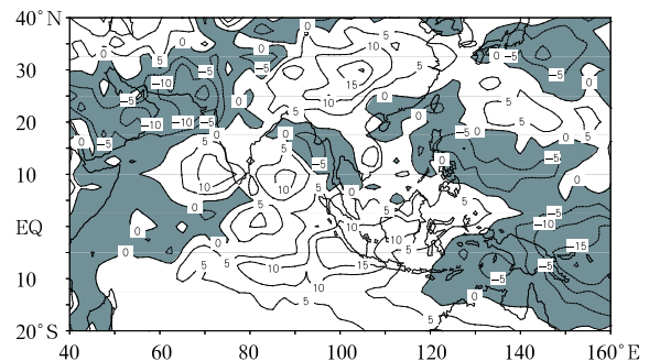
Fig. 9. The OLR anomaly field in summer 2006 ( \text{W m}^{-2} ). The climatology period is 1979–2006; shadings denote negative values.
