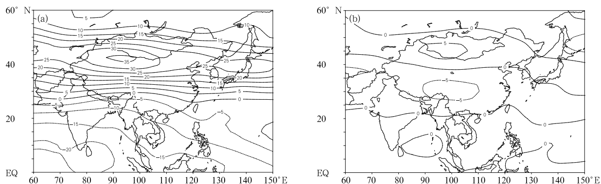
Fig. 4. The zonal wind ( \text{m s}^{-1} ) field (a) and its anomalies (b) at 200 hPa in summer 2006.
