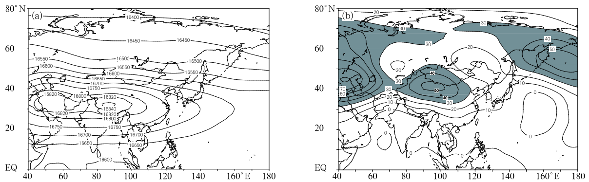
Fig. 5. The geopotential height (gpm) field (a) and its anomalies (b) at 100 hPa in summer 2006.
